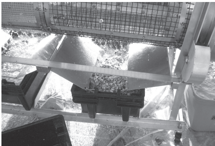
Sized oysters fall through mesh into removable bins
